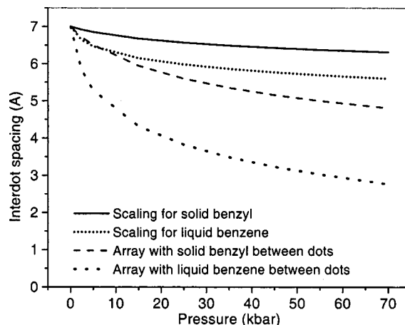
FIG. 10. Interdot separation as a function of pressure modeling the interdot medium as either solid benzyl or liquid benzene, as described in the Appendix. Also shown is how a length of 7 Å in these two media scales with pressure in the bulk. (Any phase transition in the liquid benzene is not included in these models.)
