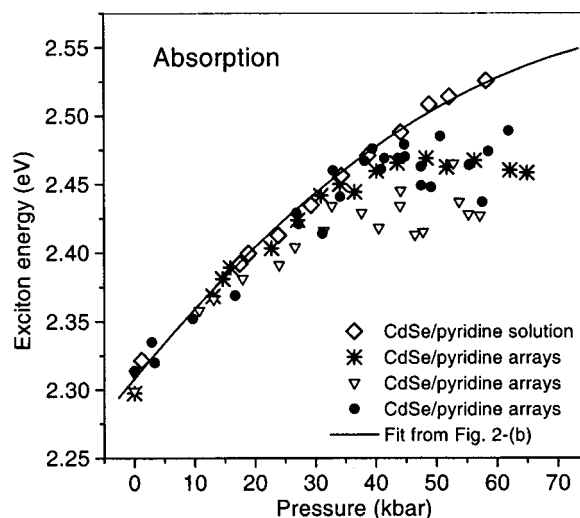
FIG. 5. The first excitonic peak energies in absorption spectra for several CdSe/pyridine runs. Note the significant difference between the solution and the array runs. Each plot has been shifted by up to \sim 10 meV so that each overlaps at 1 bar. The solid line is the fit to the exciton absorption data in (and also plotted in) Fig. 2(b).
